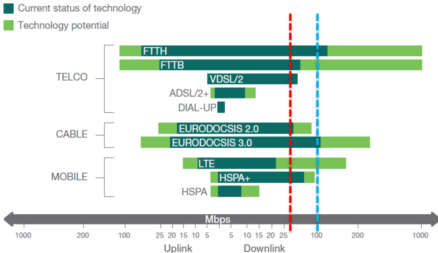
Figure 3: Typical net bit rate by technology Source: Arthur D. Little analysis
